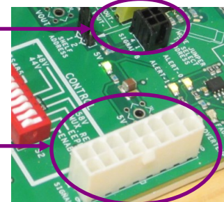
Figure 8 - Signal connector
