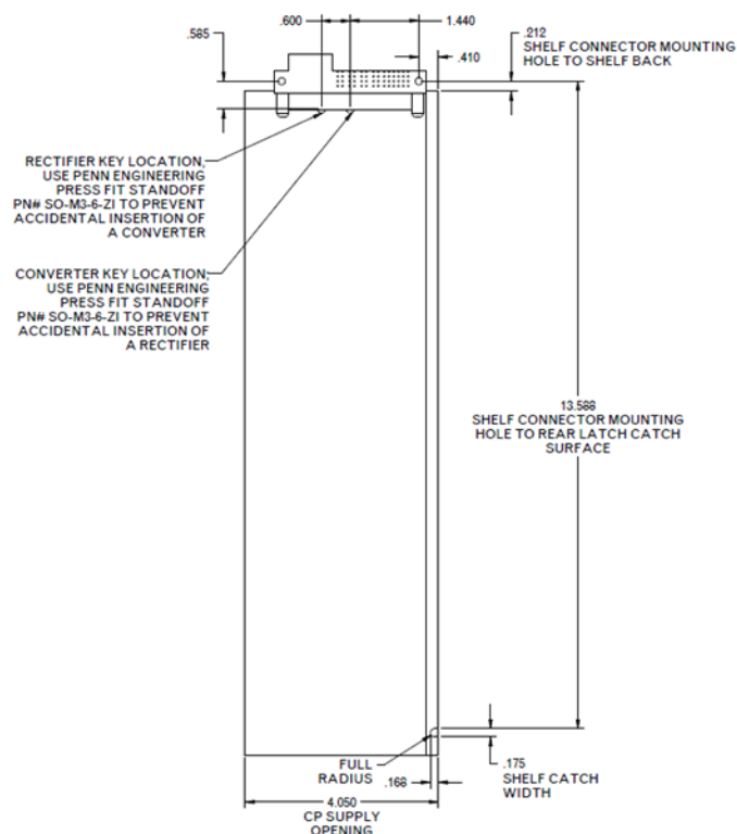
Figure 19 - Slot drawing
