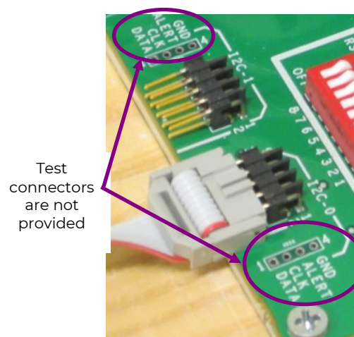
Figure 5 - Signal Connections
