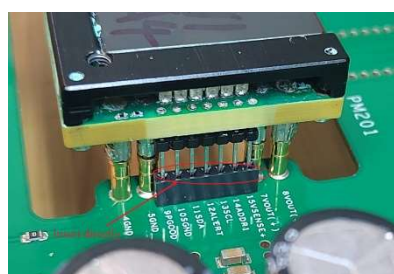
Fig. 2 Inserting Pins
