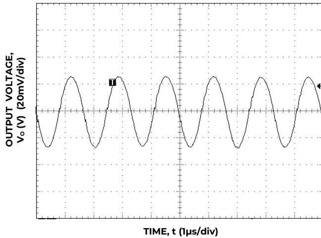
Figure 32. Typical Output Ripple and Noise, V_{IN} = 12\text{ V} , I_o = I_{o, \text{max}} .
