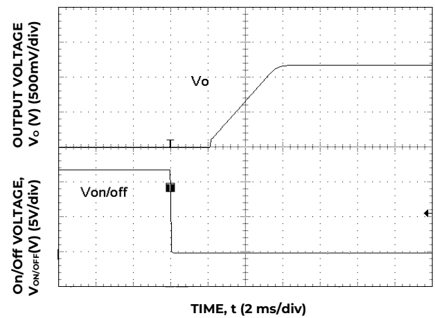
Figure 11. Typical Start-up Using On/Off Voltage ( I_o = I_{o, \text{max.}} ).
