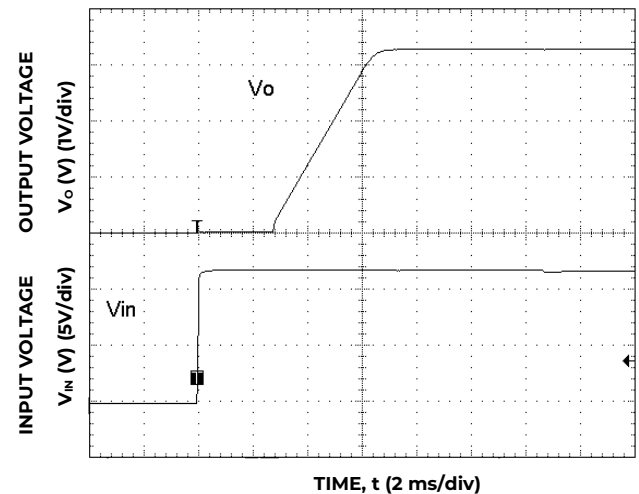
Figure 30. Typical Start-up Using Input Voltage ( V_{IN} = 12 \text{ V} , I_o = I_{o, \text{max.}} ).
