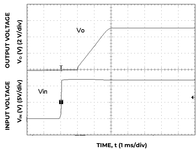
Figure 36. Typical Start-up Using Input Voltage ( V_{IN} = 12\text{ V} , I_o = I_{o, \text{max}} ).
