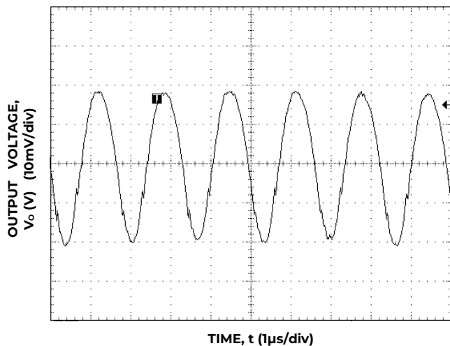
Figure 27. Typical Output Ripple and Noise, V_{IN} = 12 \text{ V} , I_o = I_{o, \text{max.}}
