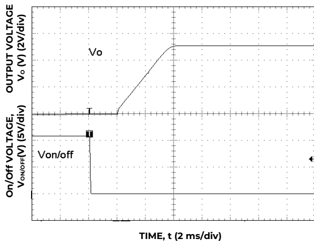
Figure 33. Typical Start-up Using On/Off Voltage ( I_o = I_{o, \text{max}} ).
