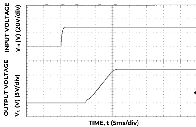
Figure 19. Typical Start-up Using Input Voltage ( V_{IN} = 28V , I_o = I_{o,max} ).
