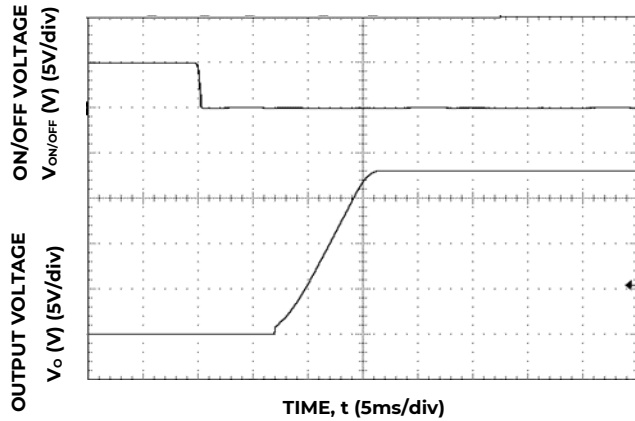
Figure 25. Typical Start-up Using On/Off Voltage ( I_o = I_{o,max} ).
