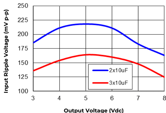
Figure 30. Input ripple voltage for various output voltages with 2x10 µF or 3x10 µF ceramic capacitors at the input (maximum load). Input voltage is 12V.
