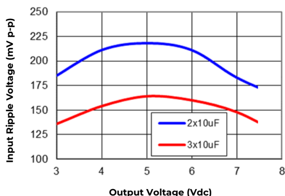
Figure 31. Input ripple voltage for various output voltages with 2x10 µF or 3x10 µF ceramic capacitors at the input (maximum load). Input voltage is 12V. (-78 version)
