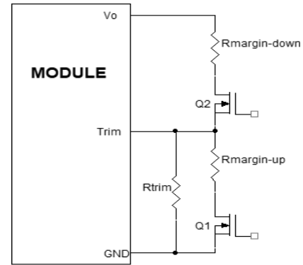
Figure 41. Circuit Configuration for margining Output voltage
