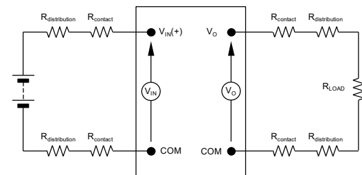
Figure 28. Output Ripple and Noise Test Setup.
