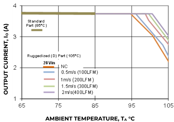
Figure 15. Derating Output Current versus Ambient Temperature and Airflow.
