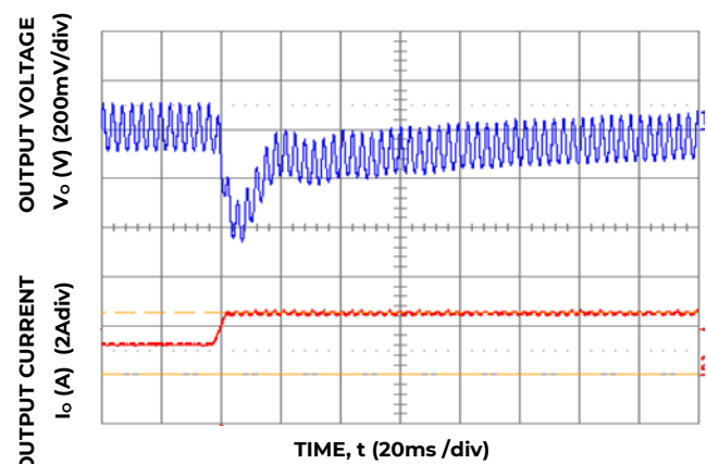
Figure 24. Transient Response to Dynamic Load Change from 50% to 100% at 28Vin, Cext - 1x10uF ceramic, CTune=150pF & RTune=220Ω
