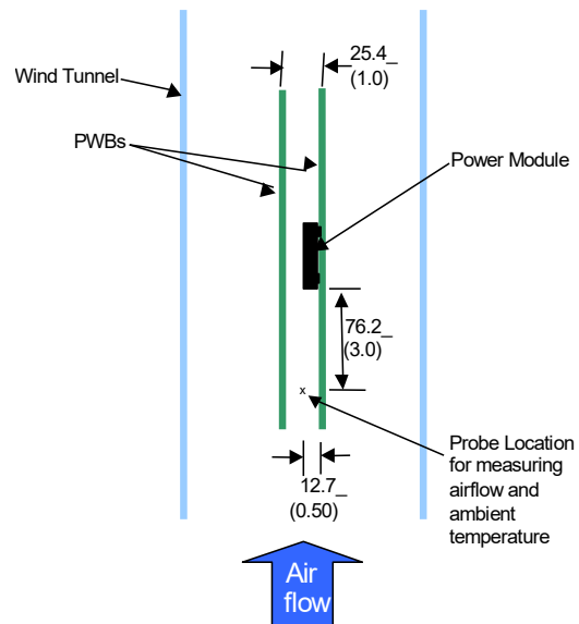
Figure 43. Thermal Test Setup.
