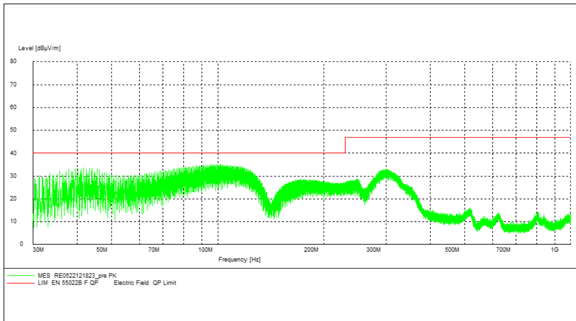
Figure 46. EMI Plot of APXW005 on evaluation board with 12V in @ 1.8 A in / 5 Vdc @ 4 A out
