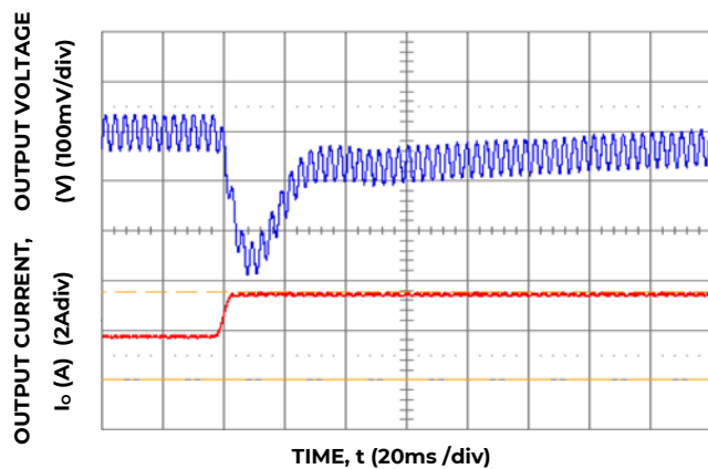
Figure 17. Transient Response to Dynamic Load Change from 50% to 100% at 28Vin, Cext - 3x10uF ceramic CTune=470pF & RTune=150Ω
