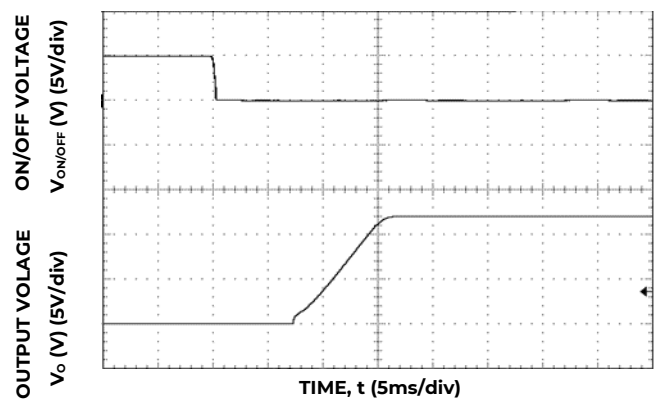
Figure 18. Typical Start-up Using On/Off Voltage ( I_O = I_{O,max} ).
