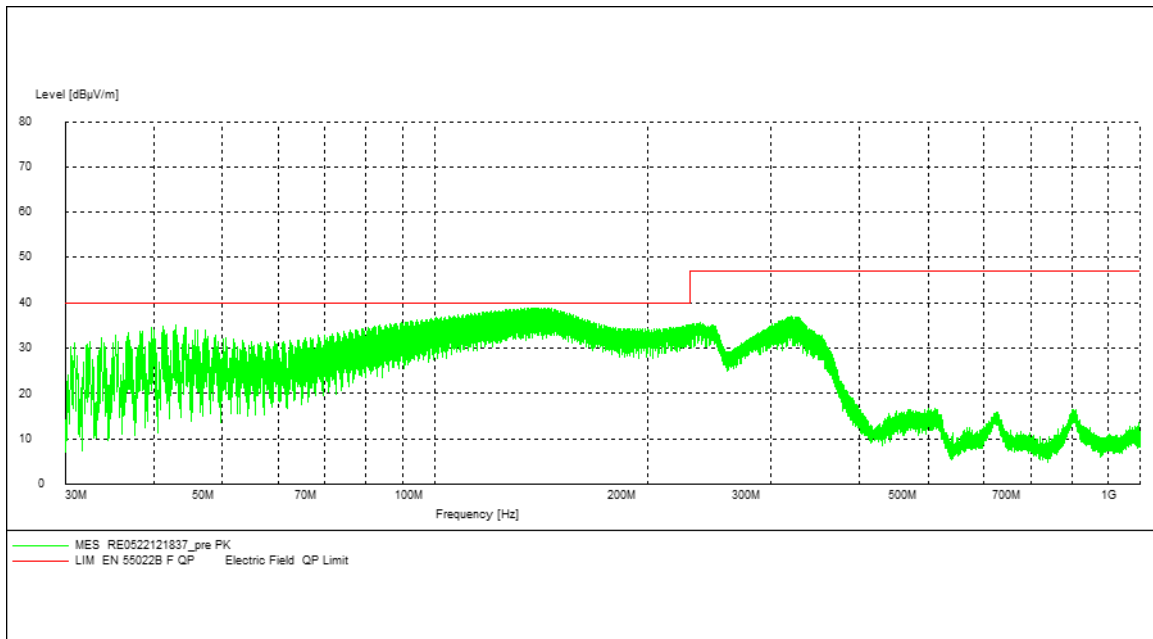
Figure 47. EMI Plot of APXW005 on evaluation board with 24 Vin @ 0.9 Ain / 5Vdc @ 4Aout
