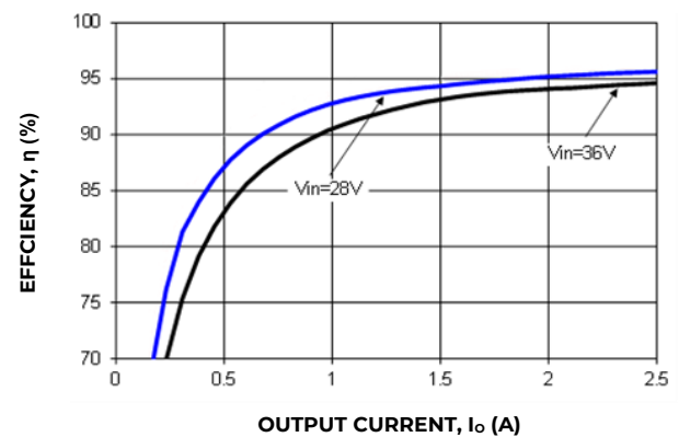
Figure 22. Converter Efficiency versus Output Current. (-78 version)
