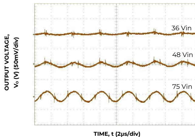
Figure 10. Typical Output Ripple and Noise at Room Temperature I_o = I_{o,max} and C_{OMin} .
