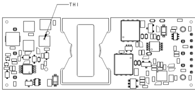
Figure 19. Location of the thermal reference temperature TH. Do not exceed 113°C.
