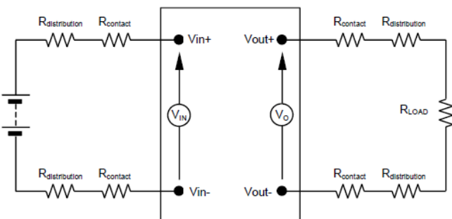
NOTE: Figure 9. Output Voltage and Efficiency Test Setup. All
