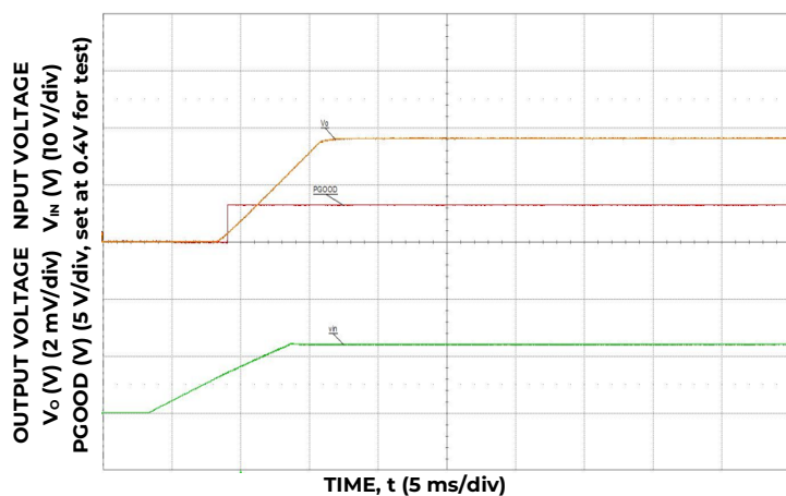
Typical Start-up Using Input Voltage (V IN = 12 V, V OUT = 3.54 V I o = I o,max ).
