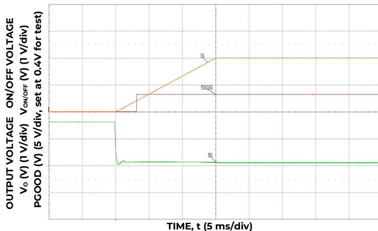
Typical Start-up Using On/Off Voltage ( I_o = I_{o,max} ).
