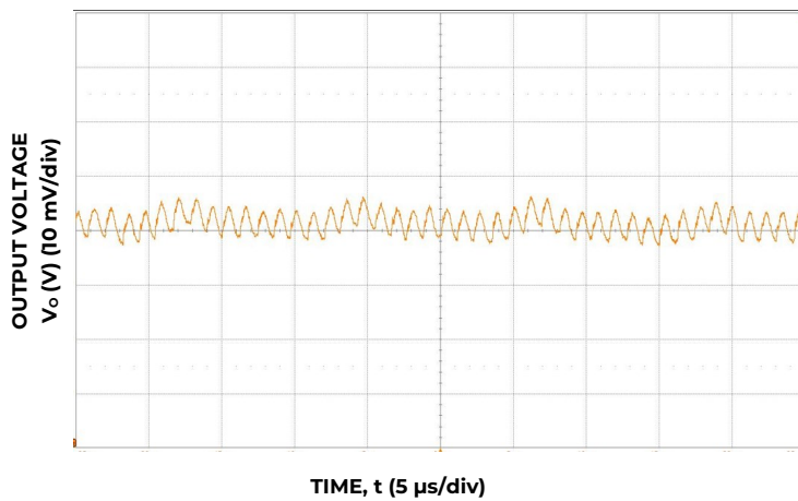
Typical output ripple, C_o=8x470\mu F+48x47\mu F+2x22\mu F+6x0.1\mu F , V_{in}=12V , I_o=I_{o,max}
