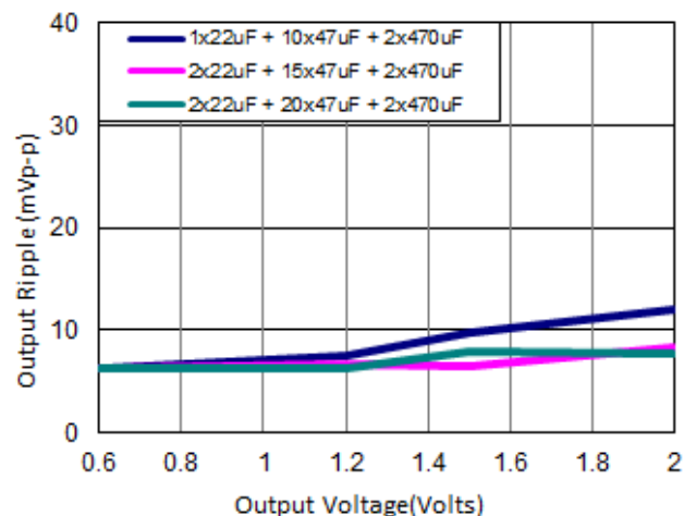
Peak to peak output ripple voltage for various output voltages with external capacitors at the output (30 A load). Input voltage is 12V.
