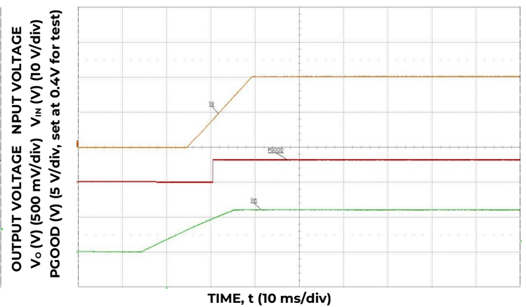
Typical Start-up Using Input Voltage ( V_{in}=12V , I_o=I_{o,max} ).
