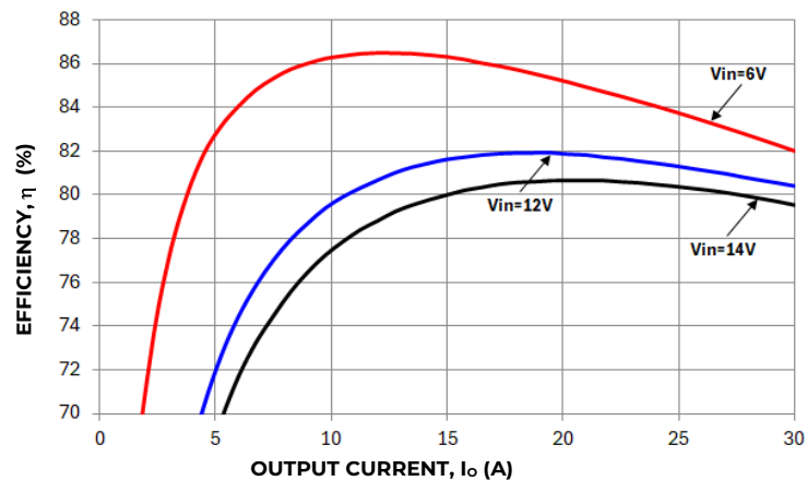
Converter Efficiency versus Output Current.
