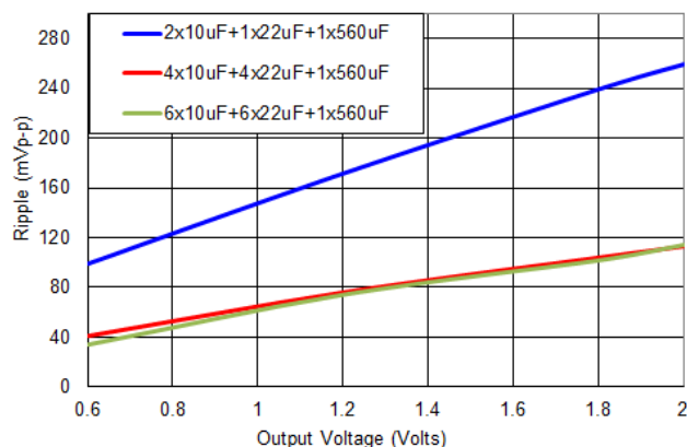
Input ripple voltage for various output voltages with three input capacitor combinations at full load. Input voltage is 12V.
