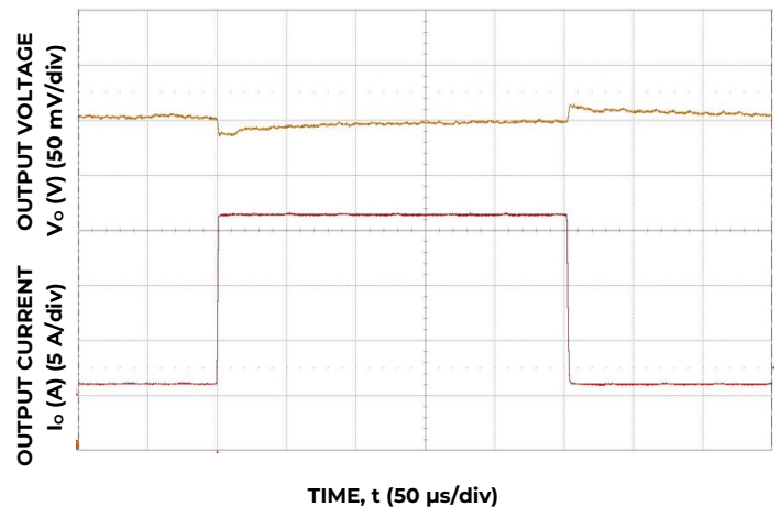
Transient response to 10 A/ \mu s Load Change from 25% to 75% at 12V in , C_o=8x470\mu F+48x47\mu F+2x22\mu F+6x0.1\mu F
