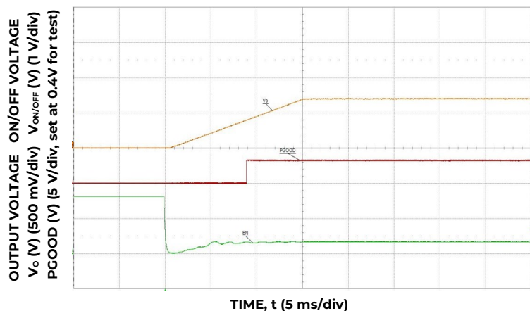
Typical Start-up Using On/Off Voltage (I o = I o,max ).
