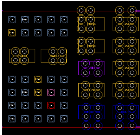
Figure 28. Example of Pad Layout with Vias.
