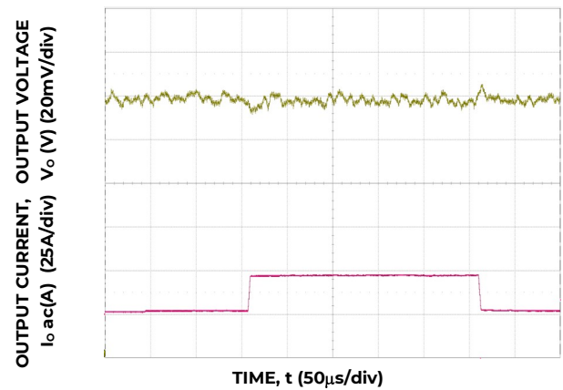
Figure 22. Trans. Resp. to 10A/μs Load Change from 25% to 75% at 12V IN , C o = 4x0.047μF + 4x0.1μF + 15x22μF + 73x47μF + 6x470μF polymer
