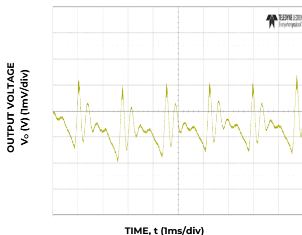
Figure 9. Typical output ripple( C_o=4 \times 0.047\mu\text{F} + 4 \times 0.1\mu\text{F} + 15 \times 22\mu\text{F} + 73 \times 47\mu\text{F} + 6 \times 470\mu\text{F} polymer, V_{in} = 12\text{V} , I_o = I_{o,max} ).
