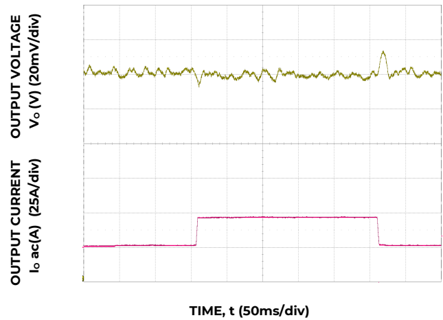
Figure 4. Trans. Resp. to 10A/μs Load Change from 25% to 75% at 12V IN , C o =4x0.047μF + 4x0.1μF + 15x22μF + 73x47μF + 6x470μF polymer
