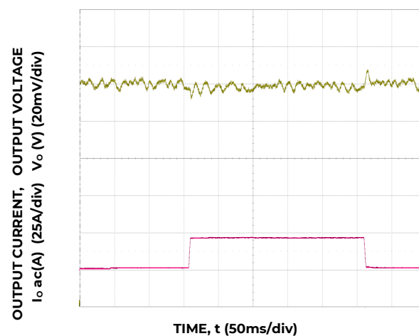
Figure 10. Trans. Resp. to 10A/μs Load Change from 25% to 75% at 12V in , C_o= 4 \times 0.047\mu\text{F} + 4 \times 0.1\mu\text{F} + 15 \times 22\mu\text{F} + 73 \times 47\mu\text{F} + 6 \times 470\mu\text{F} polymer
