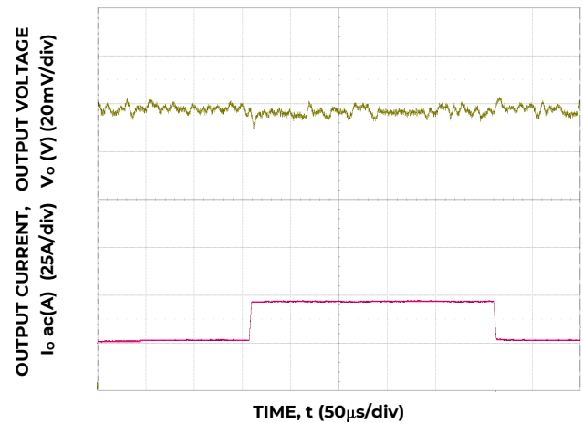
Figure 16. Trans. Resp. to 10A/μs Load Change from 25% to 75% at 12V IN , C_o = 4 \times 0.047 \mu F + 4 \times 0.1 \mu F + 15 \times 22 \mu F + 73 \times 47 \mu F + 6 \times 470 \mu F polymer
