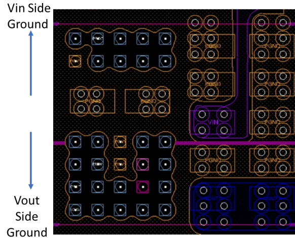
Figure 30. Example of split input-output ground
