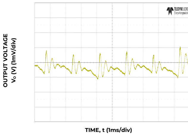
Figure 3. Typical output ripple (C o =4x0.047μF + 4x0.1μF + 15x22μF + 73x47μF + 6x470μF polymer, V IN = 12V, I o = I o,max ).
