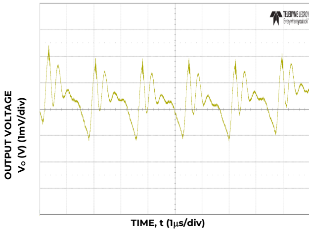
Figure 15. Typical output ripple ( C_o = 4 \times 0.047 \mu F + 4 \times 0.1 \mu F + 15 \times 22 \mu F + 73 \times 47 \mu F + 6 \times 470 \mu F polymer, V_{IN} = 12V , I_o = I_{o,max} ).
