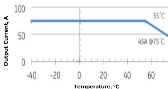
Rated Output Current (at V_{in} > 175V_{ac} )
