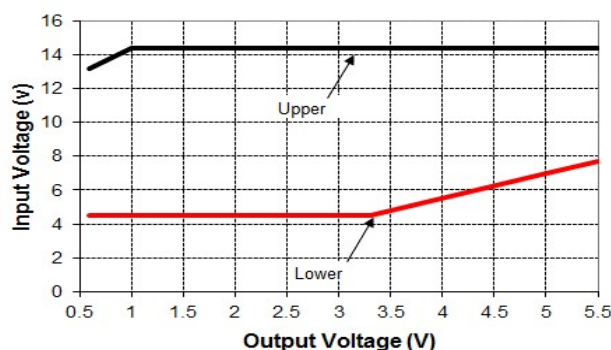
Figure 41. Output Voltage vs. Input Voltage Set Point Area plot showing limits where the output voltage can be set for different input voltages.
