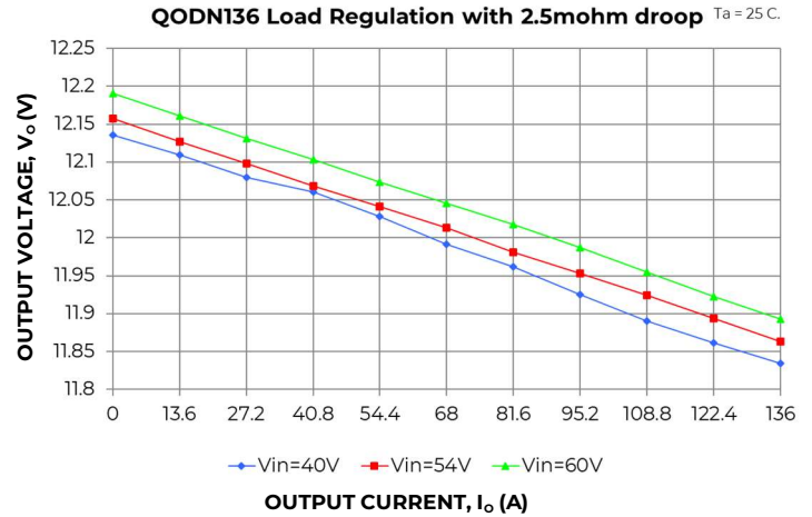
Figure 8. Typical Output Voltage Regulation vs Output Current, with droop
