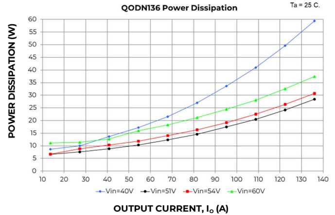
Figure 2. Power Dissipation versus Output Current
