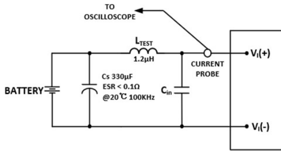
Figure 13. Input Ripple Current Test Setup.
