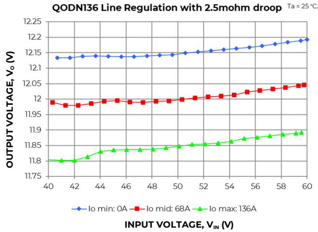
Figure 7. Typical Output Voltage Regulation vs Input Voltage, with droop
