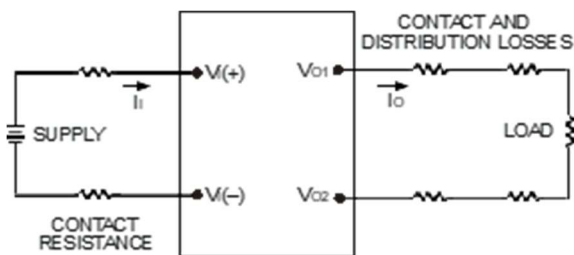
Figure 15. Output Voltage and Efficiency Test Setup.
