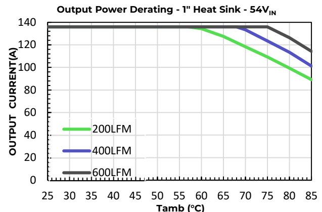
Figure 21. Maximum Output Current Derating for the QODN136A0B base plate module with 1 inch height heatsink; Airflow Direction for V_{IN}^- + to V_{IN}^+ -orientation; V_{IN} = 54\text{V} .
