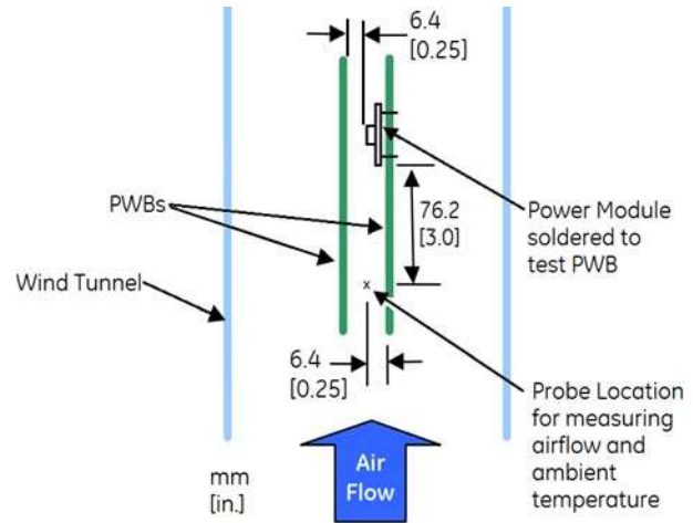
Figure 19. Thermal Test Setup
