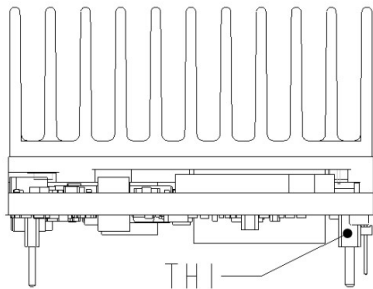
Figure 18. Location of the thermal reference temperature TH1 for base plate module with 1 inch height heatsink CC848795914
