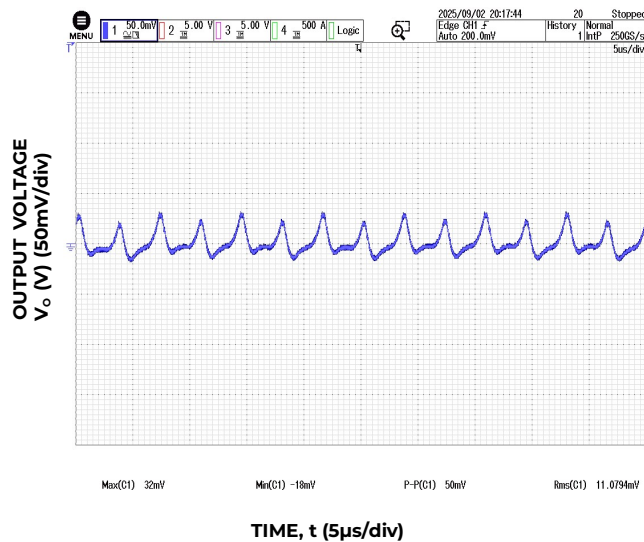
Figure 3. Typical output ripple and noise ( C_o = 250\mu\text{F} Ceramic + 3900\mu\text{F} PosCap Oscon, V_{in} = 54\text{V} , I_o = I_{o,max} )
