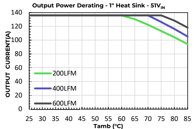
Figure 20. Maximum Output Current Derating for the QODN136A0B base plate module with 1 inch height heatsink; Airflow Direction for V_{IN}^- + to V_{IN}^+ -orientation; V_{IN} = 51\text{V} .
