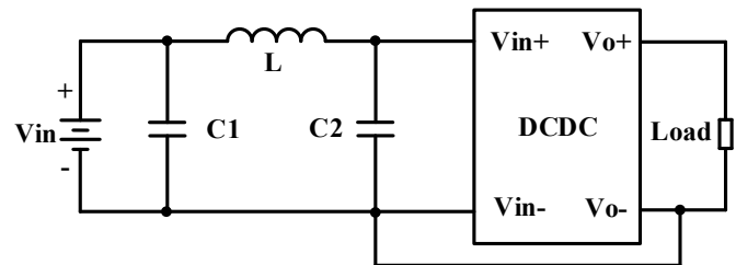
Figure 12. Optional external filter for Class A
