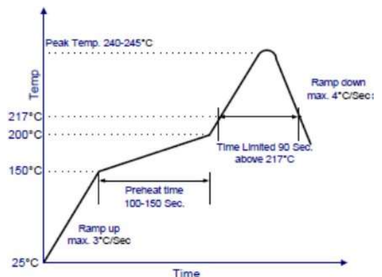
Figure 22. Recommended linear reflow profile using Sn/Ag/Cu solder.
