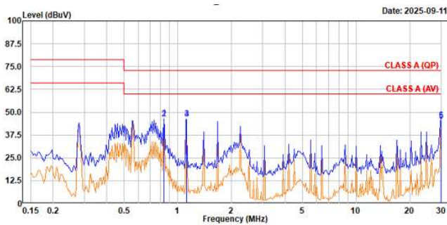
Figure 11. EMC test results
