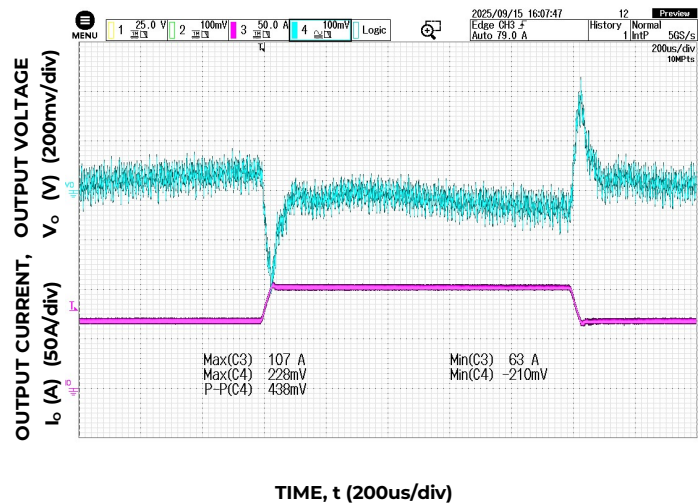
Figure 4. Dynamic Load Response, dI_o/dt=1\text{A}/\mu\text{s} ; V_{in}=54\text{V} ; T_a=25^\circ\text{C} ; Load Change from I_o = 50\% to 75\% of I_{o,max} ; C_o = 250\mu\text{F} Ceramic + 3900\mu\text{F} PosCap Oscon
