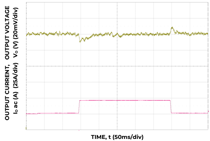
Figure 16. Trans. Resp. to 10A/μs Load Change from 25% to 75% at 12VIN, C_o = 4 \times 0.047\mu\text{F} + 4 \times 0.1\mu\text{F} + 15 \times 22\mu\text{F} + 73 \times 47\mu\text{F} + 6 \times 470\mu\text{F} polymer
