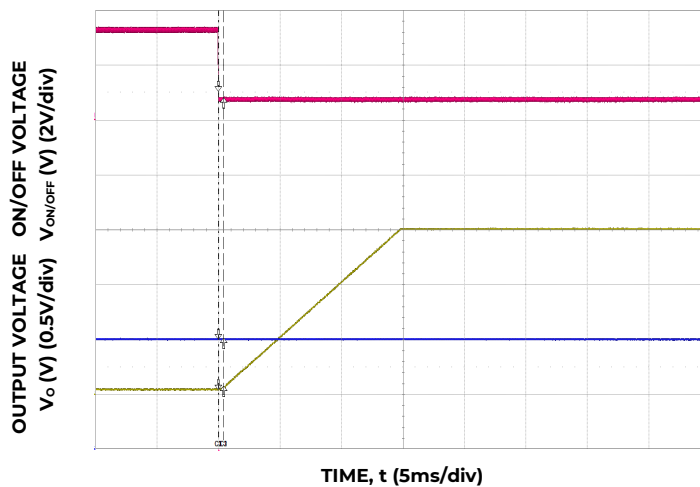
Figure 17. Typical Start-up Using On/Off Voltage ( I_o = I_{o\text{max}} ).
