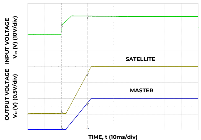
Figure 18. Typical Start-up Using Input Voltage ( V_{IN} = 12\text{V} , I_o = I_{o\text{max}} ).
