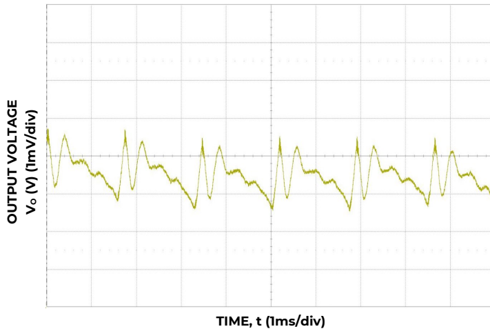
Figure 9. Typical output ripple ( C_o=4 \times 0.047\mu\text{F} + 4 \times 0.1\mu\text{F} + 15 \times 22\mu\text{F} + 73 \times 47\mu\text{F} + 6 \times 470\mu\text{F} polymer, V_{IN} = 12\text{V} , I_o = I_{o,max} ).
