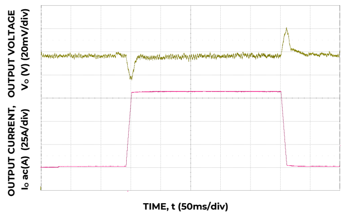
Figure 22. Trans. Resp. to 100A/μs Load Change from 25% to 75% at 12V IN , C o =4x0.047μF + 4x0.1μF + 15x22μF + 73x47μF + 6x470μF polymer
