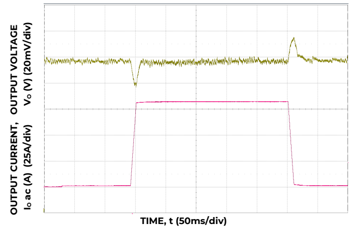
Figure 16. Trans. Resp. to 100A/μs Load Change from 25% to 75% at 12V IN , C_o=4\times0.047\mu\text{F}+4\times0.1\mu\text{F}+15\times22\mu\text{F}+73\times47\mu\text{F}+6\times470\mu\text{F} polymer
