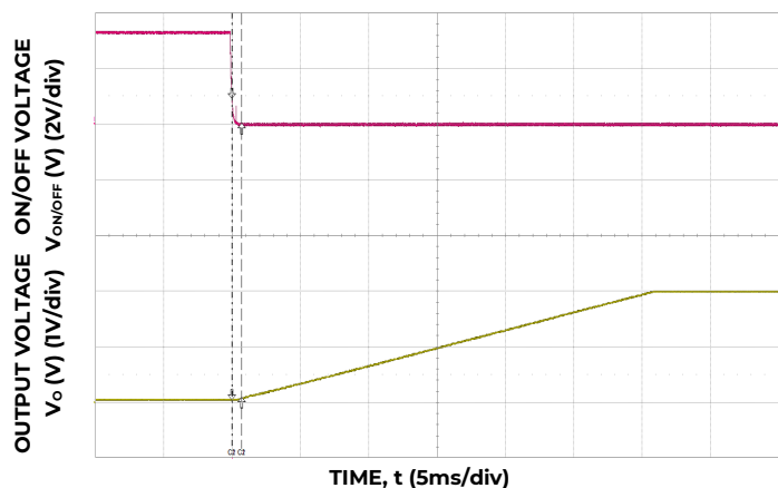
Figure 23. Typical Start-up Using On/Off Voltage (I o = I o, max ).
