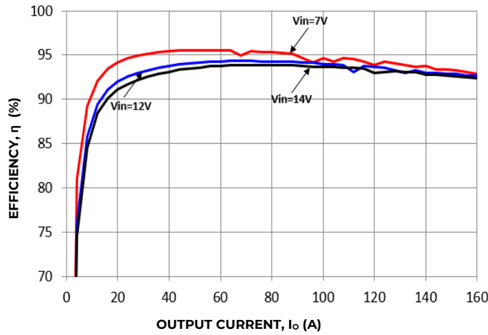
Figure 13. Converter Efficiency versus Output Current.
