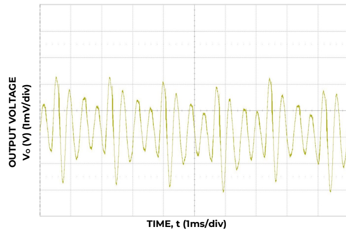
Figure 15. Typical output ripple ( C_o=4\times0.047\mu\text{F}+4\times0.1\mu\text{F}+15\times22\mu\text{F}+73\times47\mu\text{F}+6\times470\mu\text{F} polymer, V_{IN}=12\text{V} , I_o=I_{o, \text{max}} ).
