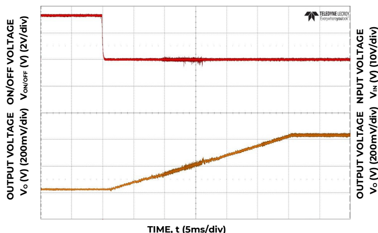
Figure 5. Typical Start-up Using On/Off Voltage ( I_o = I_{o,max} ).
