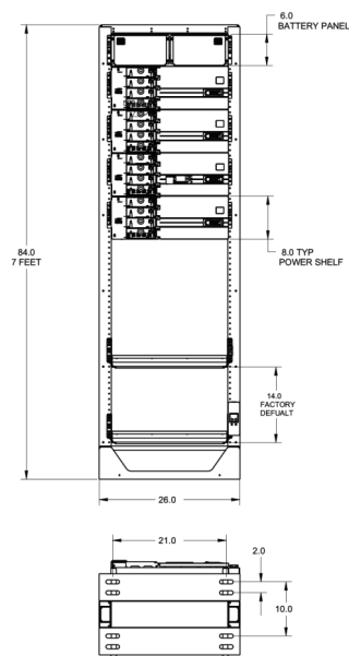
7ft High relay rack for mounting 23" wide equipment
