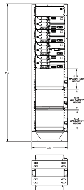
7ft relay rack for mounting 19" wide equipment
