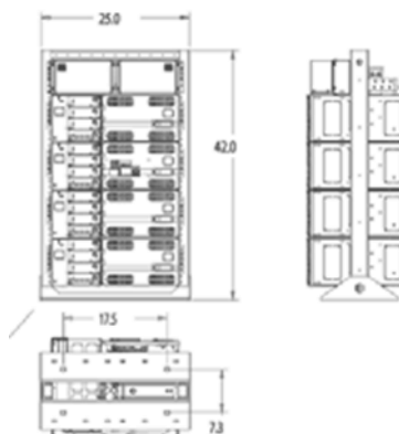
42" high relay rack for mounting 23" wide equipment on a ½ height battery stand or battery stack
